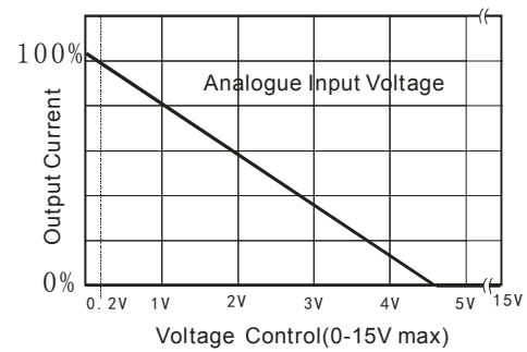
(Figure 8) Output current VS analogue input voltage
