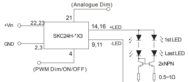
(Figure 4) Parallel-series Application
