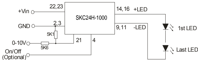
(Figure 7) Analogue dimming circuit
