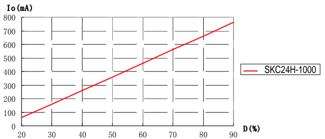
(Figure 6) Output current VS Pulse width of the PWM signal ( f=200Hz )
