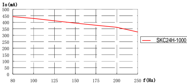
(Figure 5) PWM Frequency VS Output current( D=50\% )
