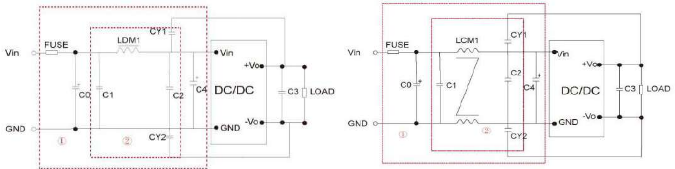
3.3VDC、5VDC Output (Figure 3)
