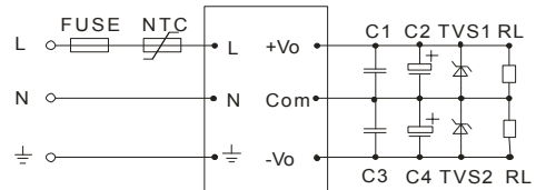
Figure 2: SLH**-10A** (Dual Output)
