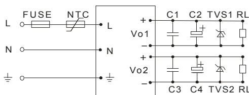
Figure 3: SLH**-10D** (Isolate Twin Output)
