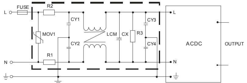
Figure 6: SLH05-25 series Recommended circuit for application require higher EMC standard (external circuit output same as above)
