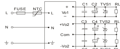
Figure 4: SLH**-10C** (Triple Output)
